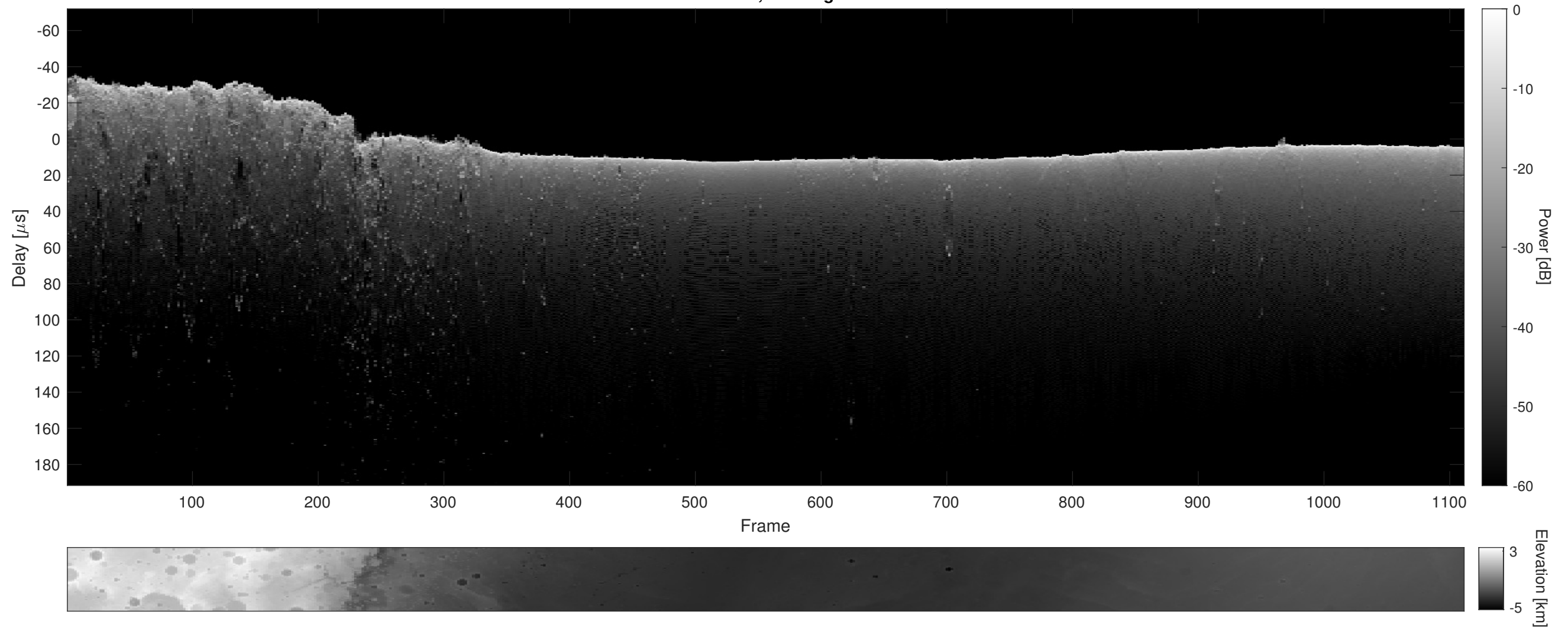
Orbit 22712, Cluttergram
