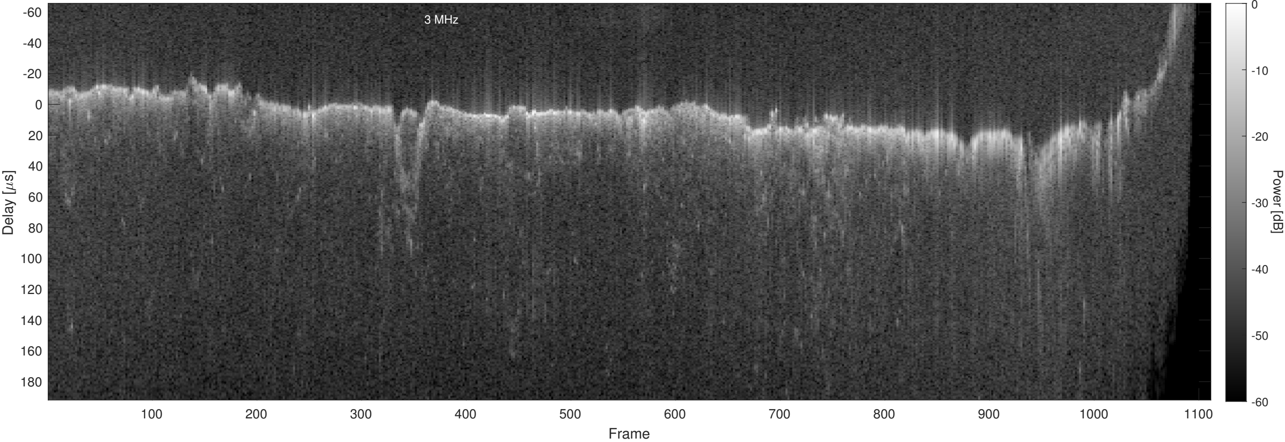
Orbit 22713, Chapman, No Window, Channel 2
