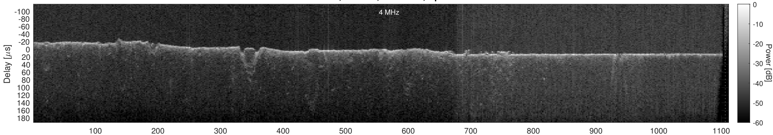
Orbit 22713, Cluttergram
