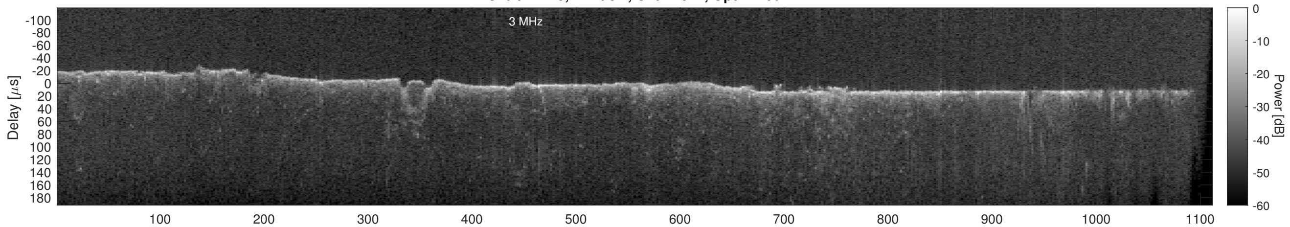
Orbit 22713, Cluttergram
