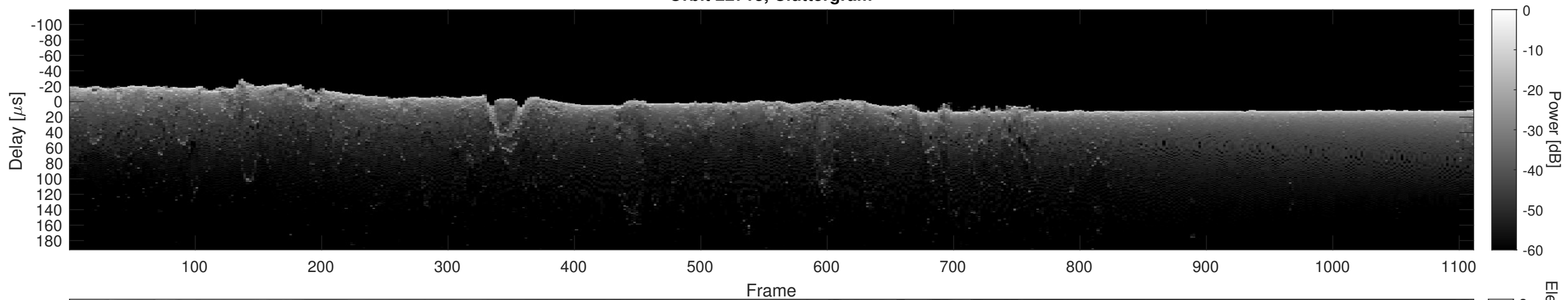
Orbit 22713, Cluttergram
