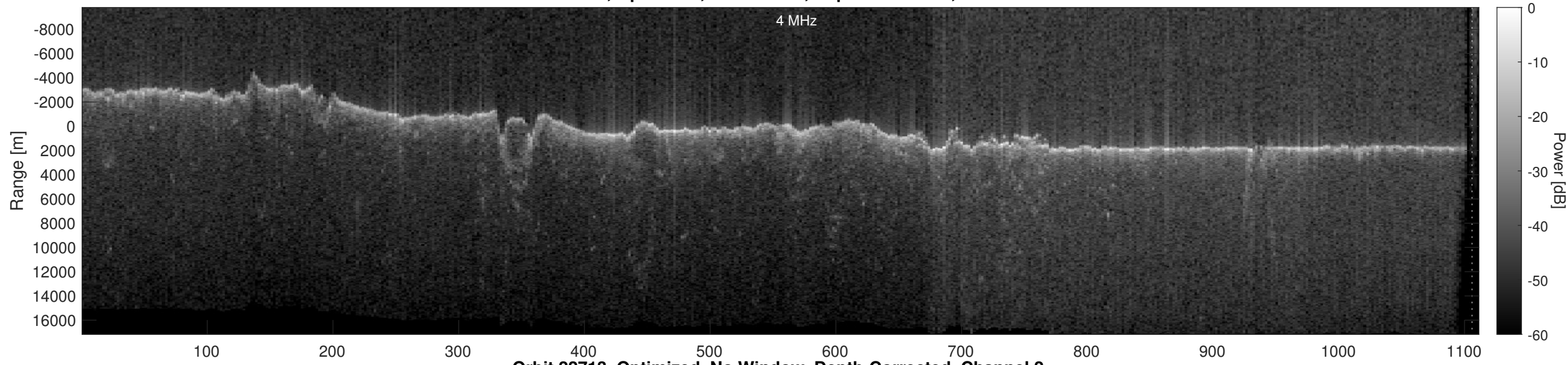
Orbit 22713, Optimized, No Window, Depth-Corrected, Channel 2
