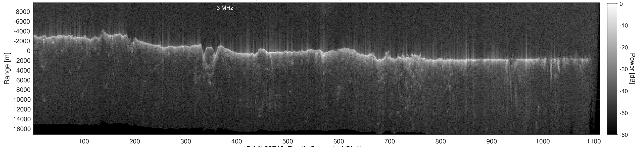
Orbit 22713, Depth-Corrected Cluttergram
