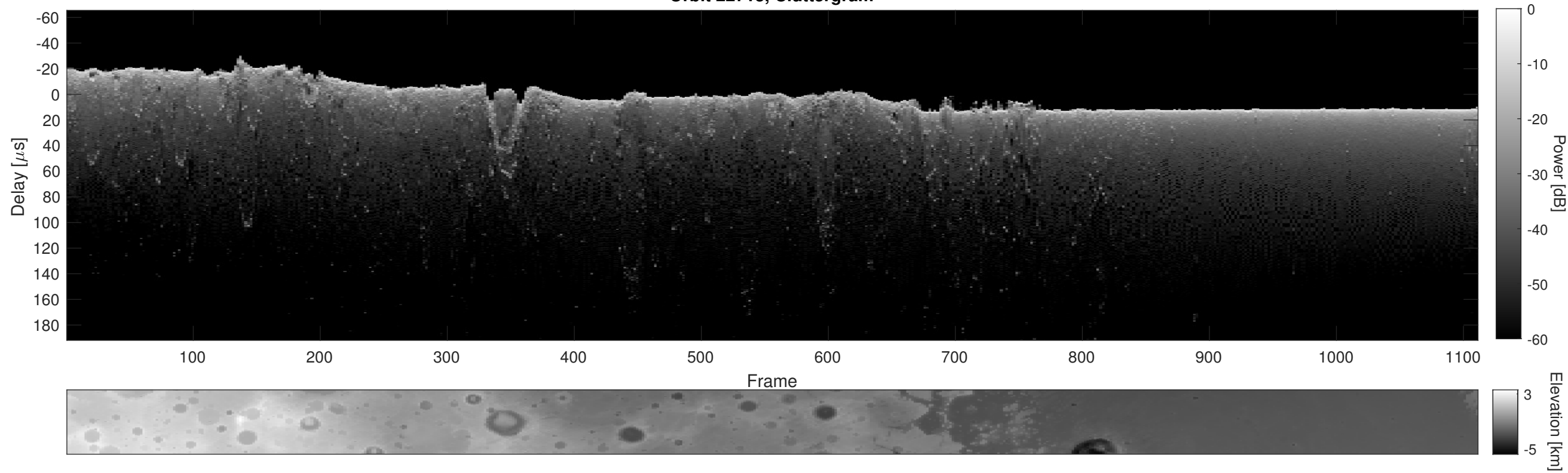
Orbit 22713, Cluttergram
