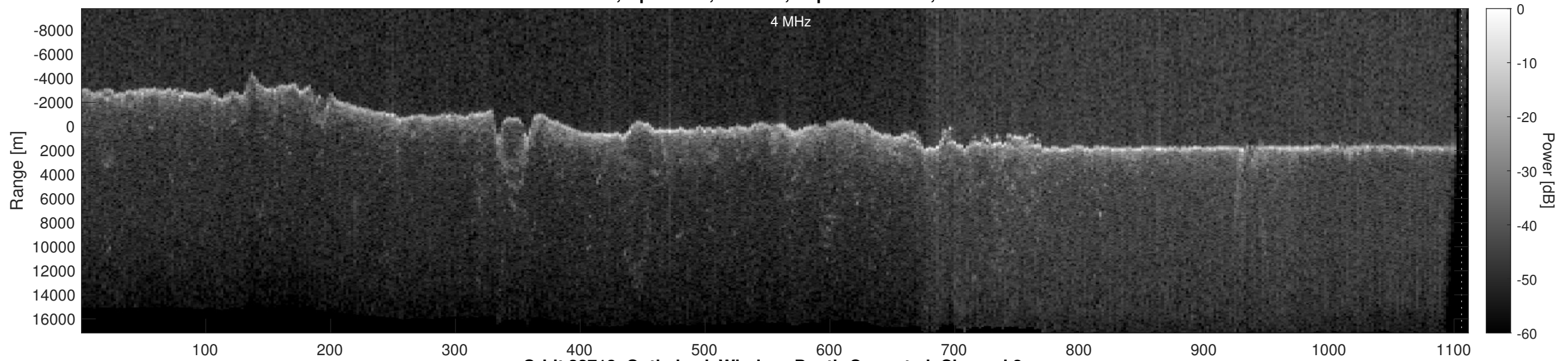
Orbit 22713, Optimized, Window, Depth-Corrected, Channel 2
