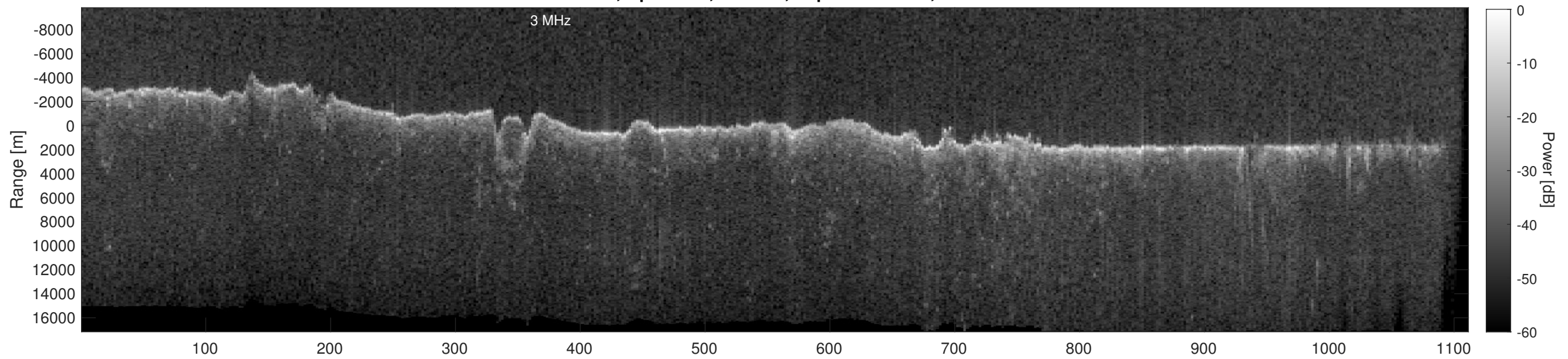
Orbit 22713, Depth-Corrected Cluttergram
