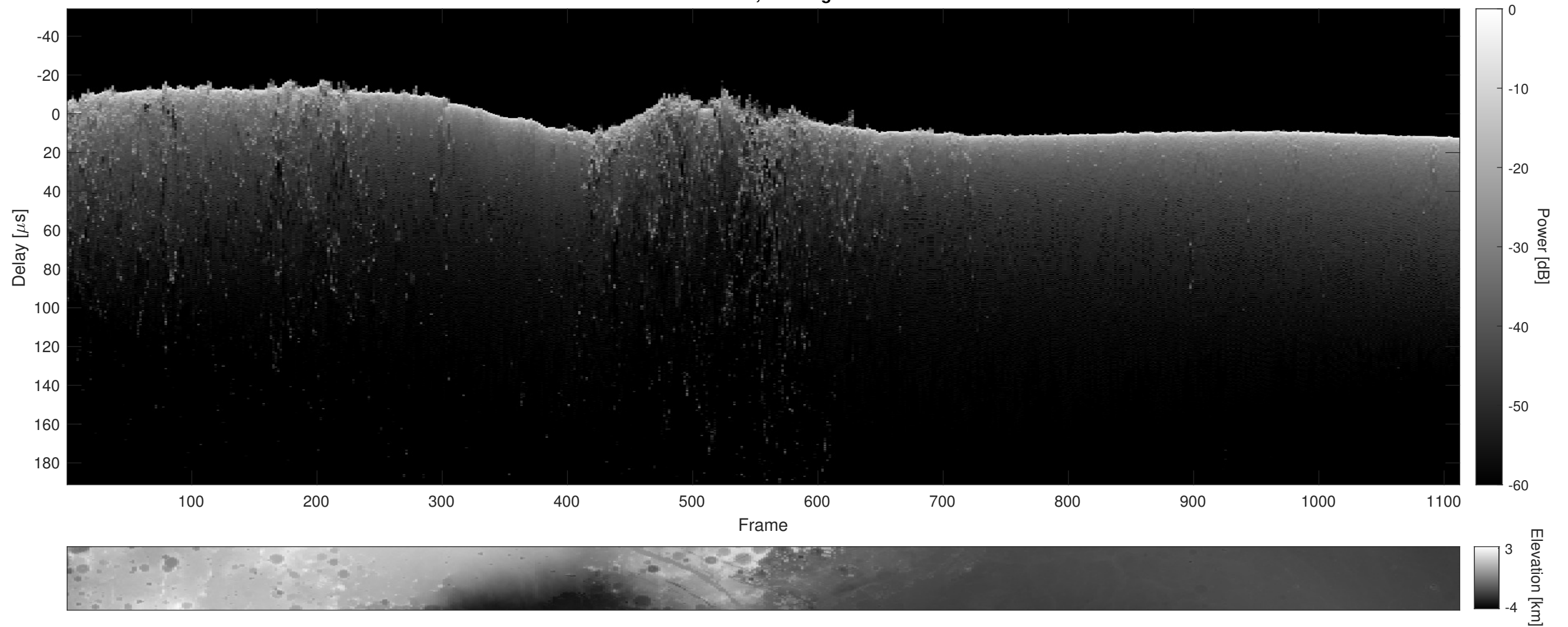
Orbit 22716, Cluttergram
