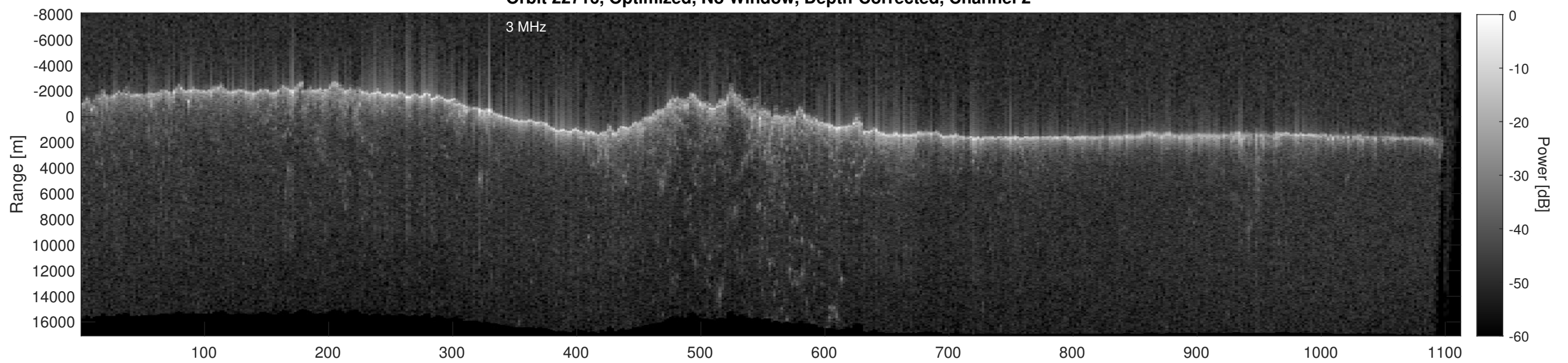
Orbit 22716, Depth-Corrected Cluttergram
