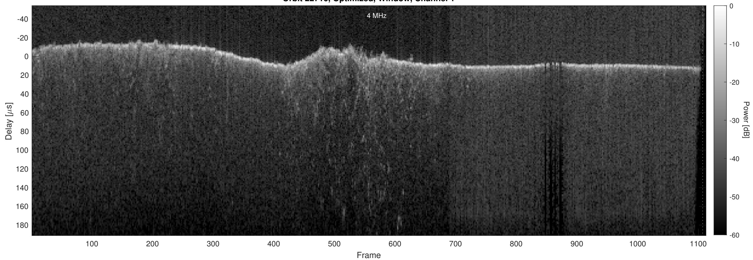
Orbit 22716, Optimized, Window, Channel 2
