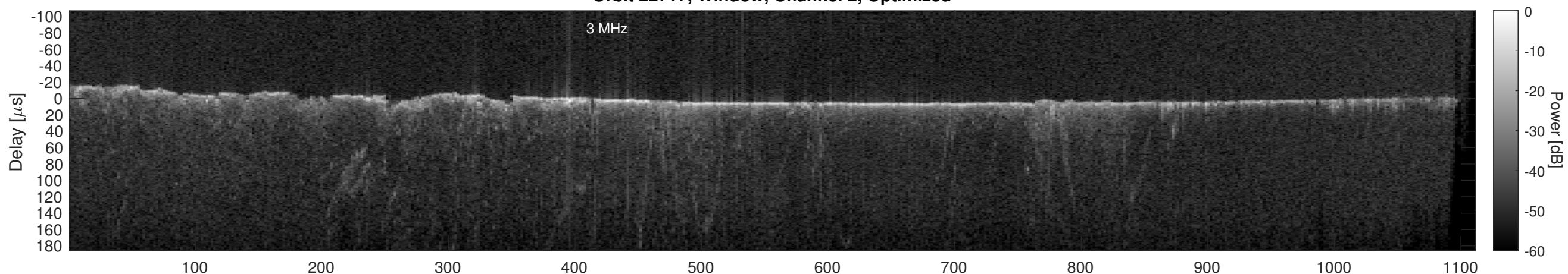
Orbit 22717, Cluttergram
