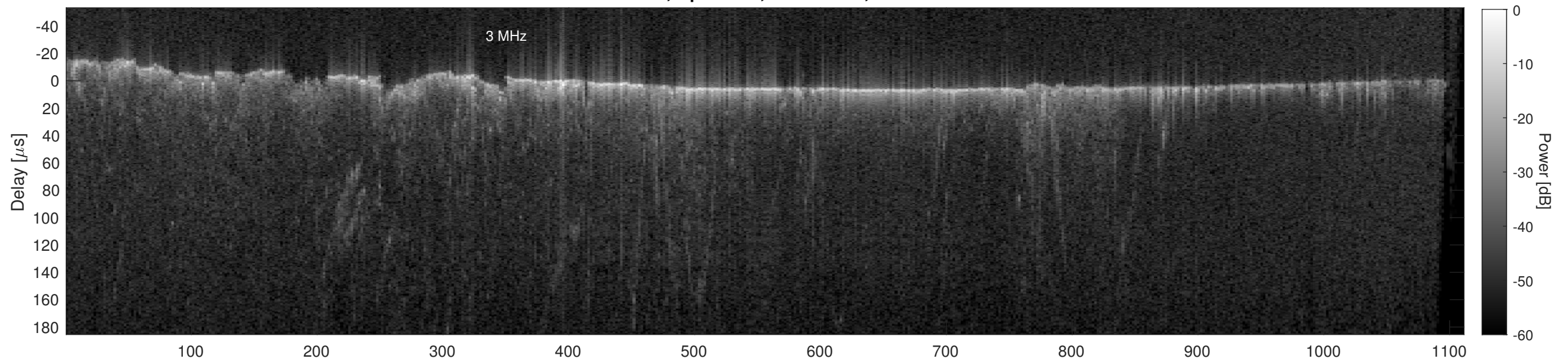
Orbit 22717, Cluttergram
