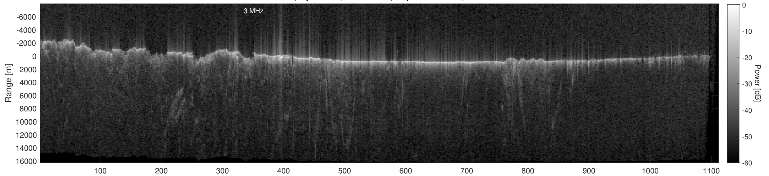
Orbit 22717, Depth-Corrected Cluttergram
