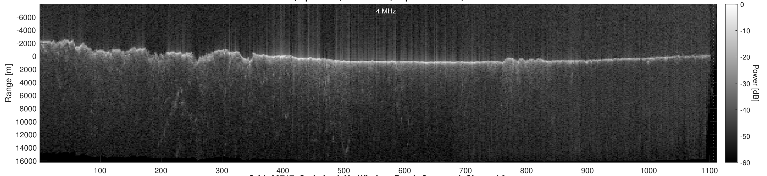
Orbit 22717, Optimized, No Window, Depth-Corrected, Channel 2
