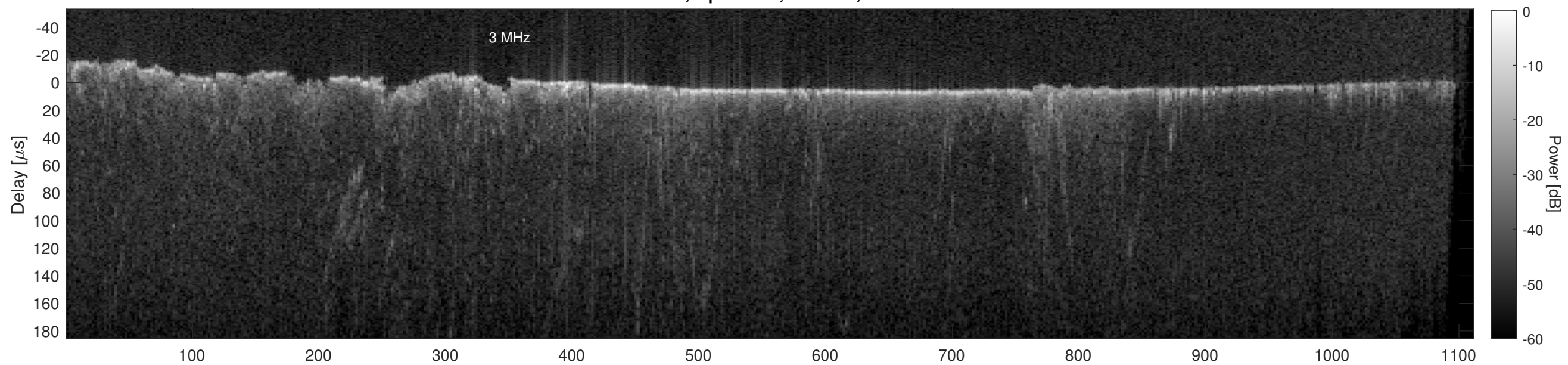
Orbit 22717, Cluttergram
