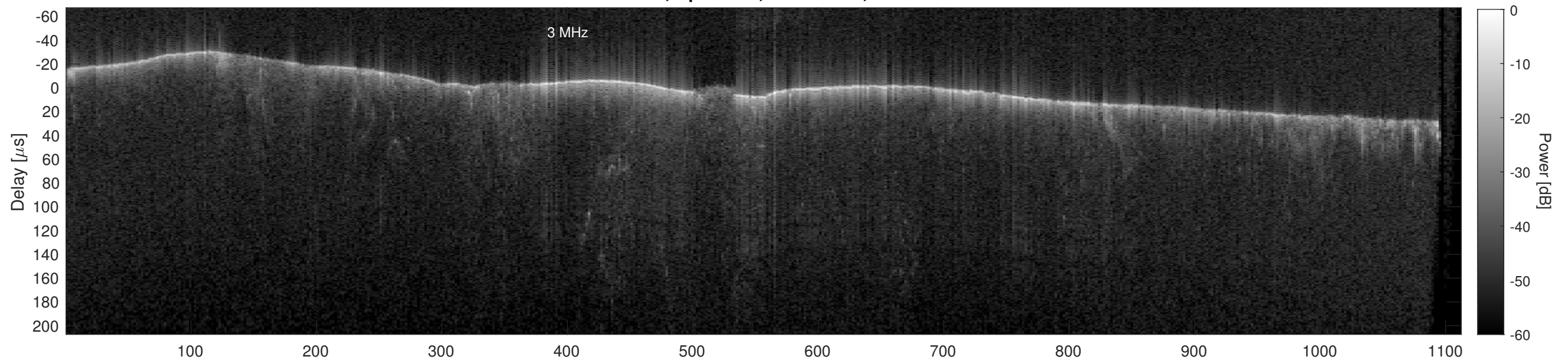
Orbit 22718, Cluttergram
