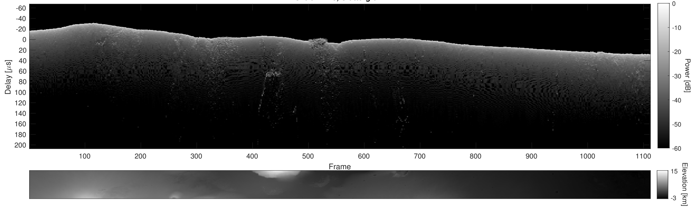
Orbit 22718, Cluttergram
