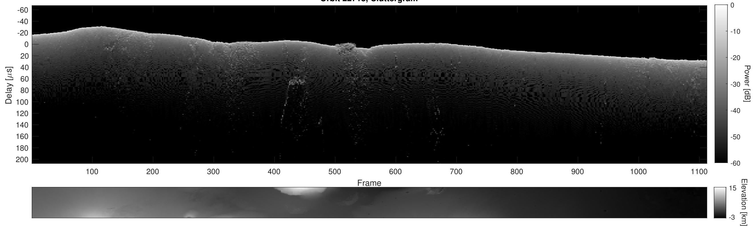
Orbit 22718, Cluttergram
