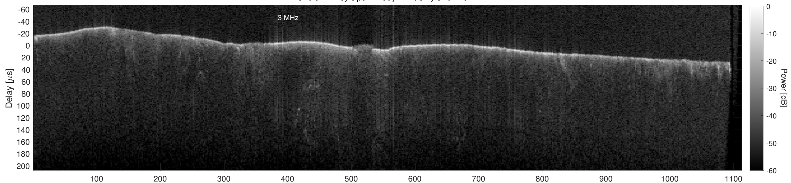
Orbit 22718, Cluttergram
