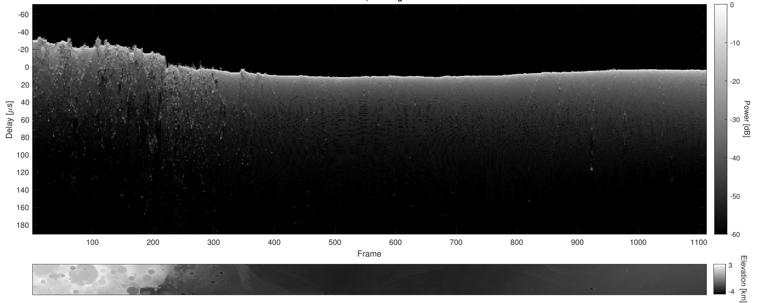
Orbit 22719, Cluttergram
