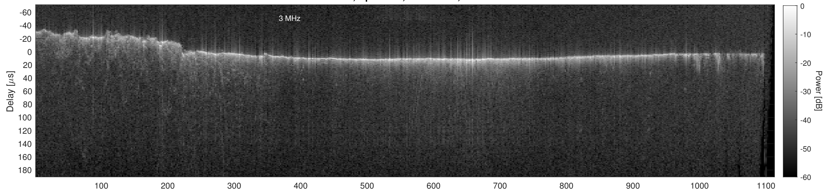
Orbit 22719, Cluttergram
