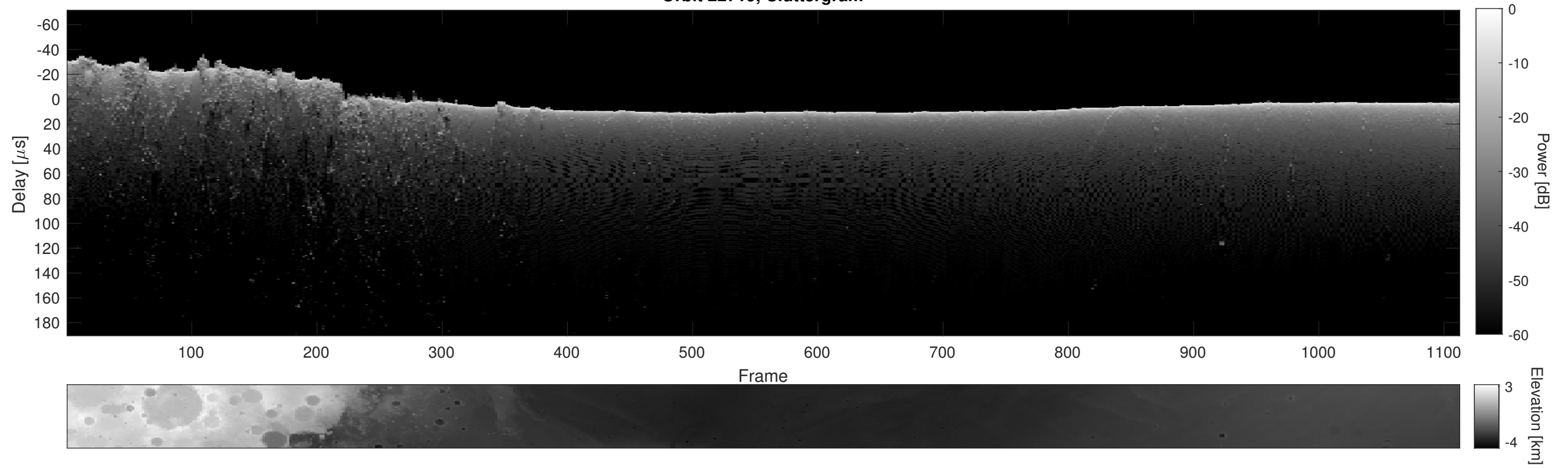
Orbit 22719, Cluttergram
