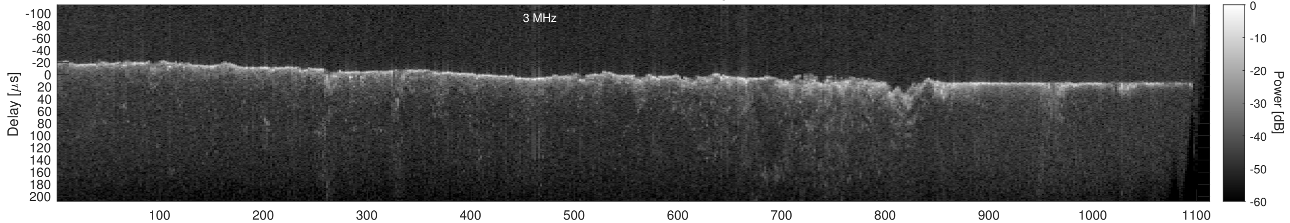
Orbit 22720, Cluttergram
