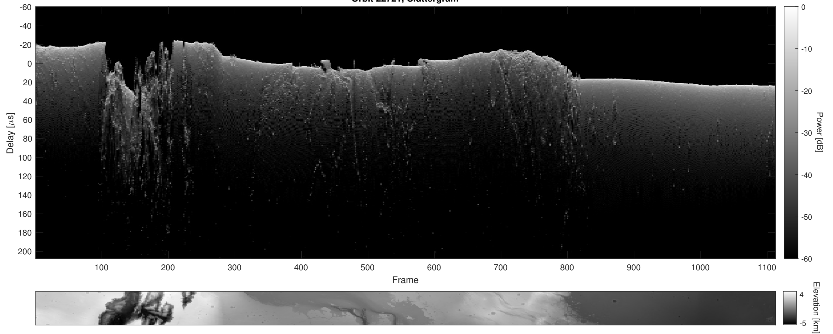
Orbit 22721, Cluttergram
