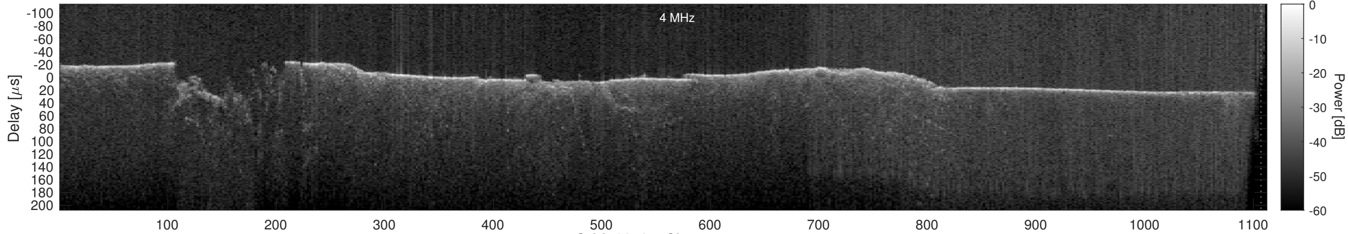
Orbit 22721, Cluttergram
