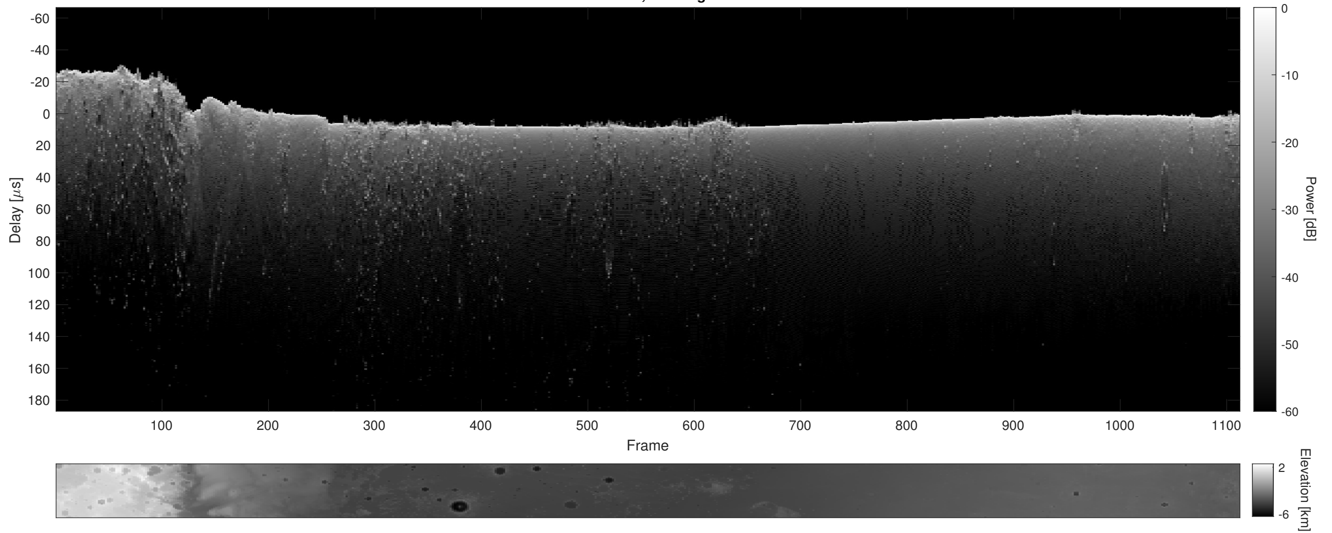
Orbit 22722, Cluttergram
