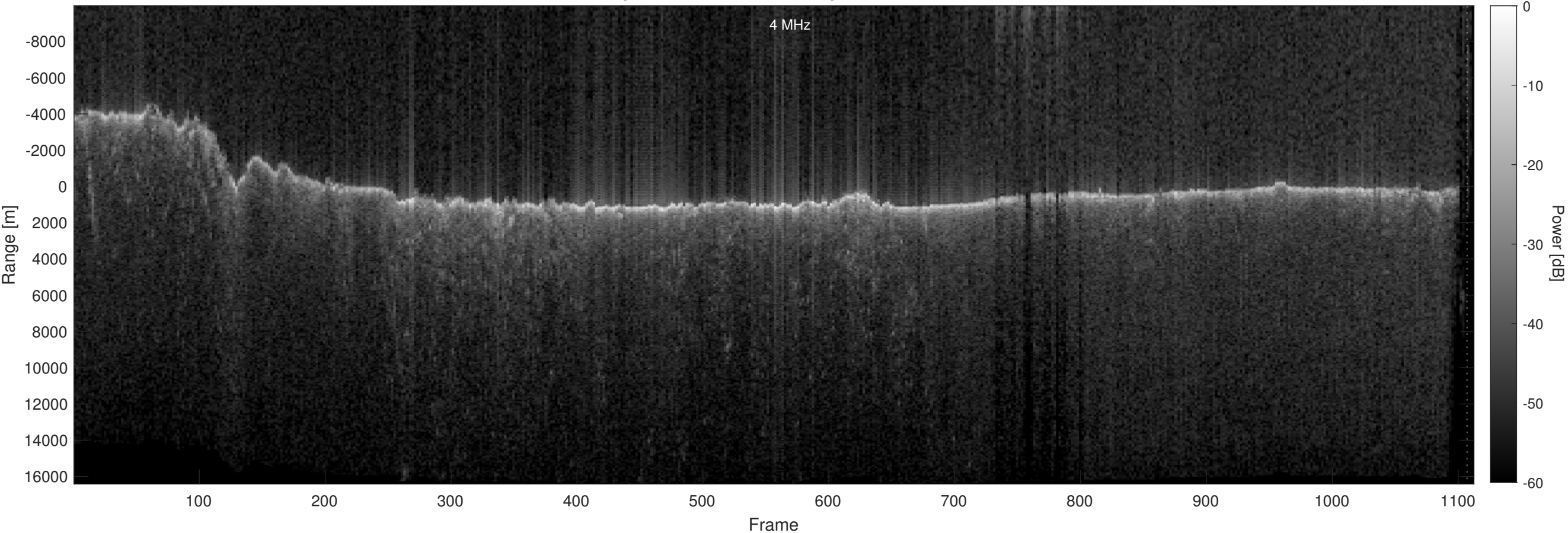
Orbit 22722, Optimized, No Window, Depth-Corrected, Channel 2
