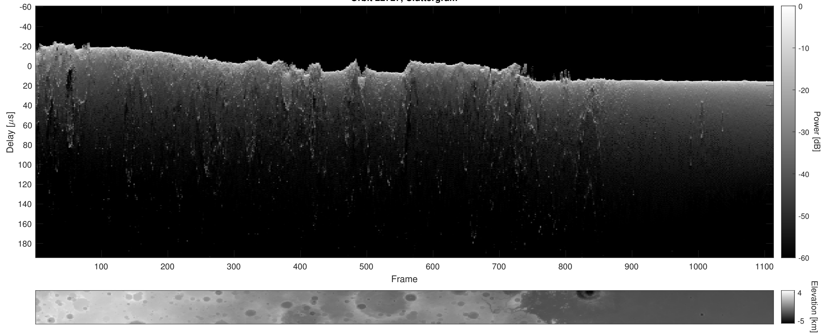
Orbit 22727, Cluttergram
