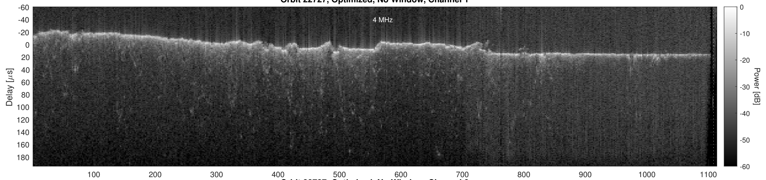
Orbit 22727, Optimized, No Window, Channel 2
