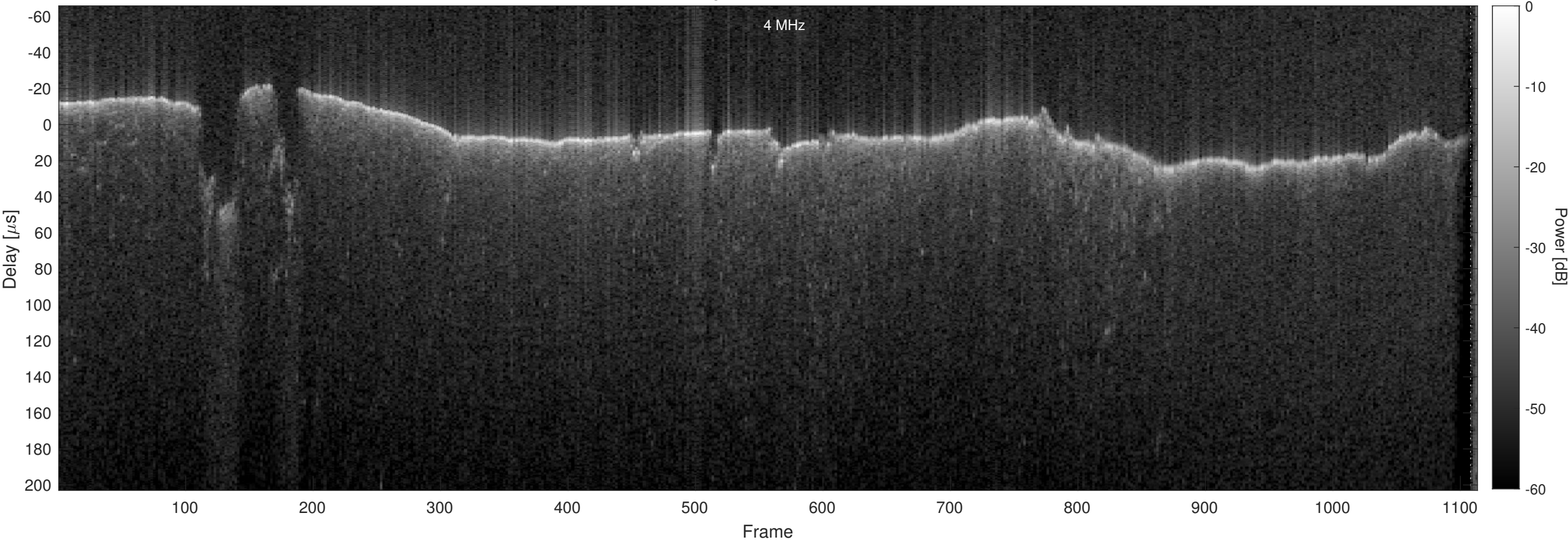
Orbit 22728, Chapman, No Window, Channel 2
