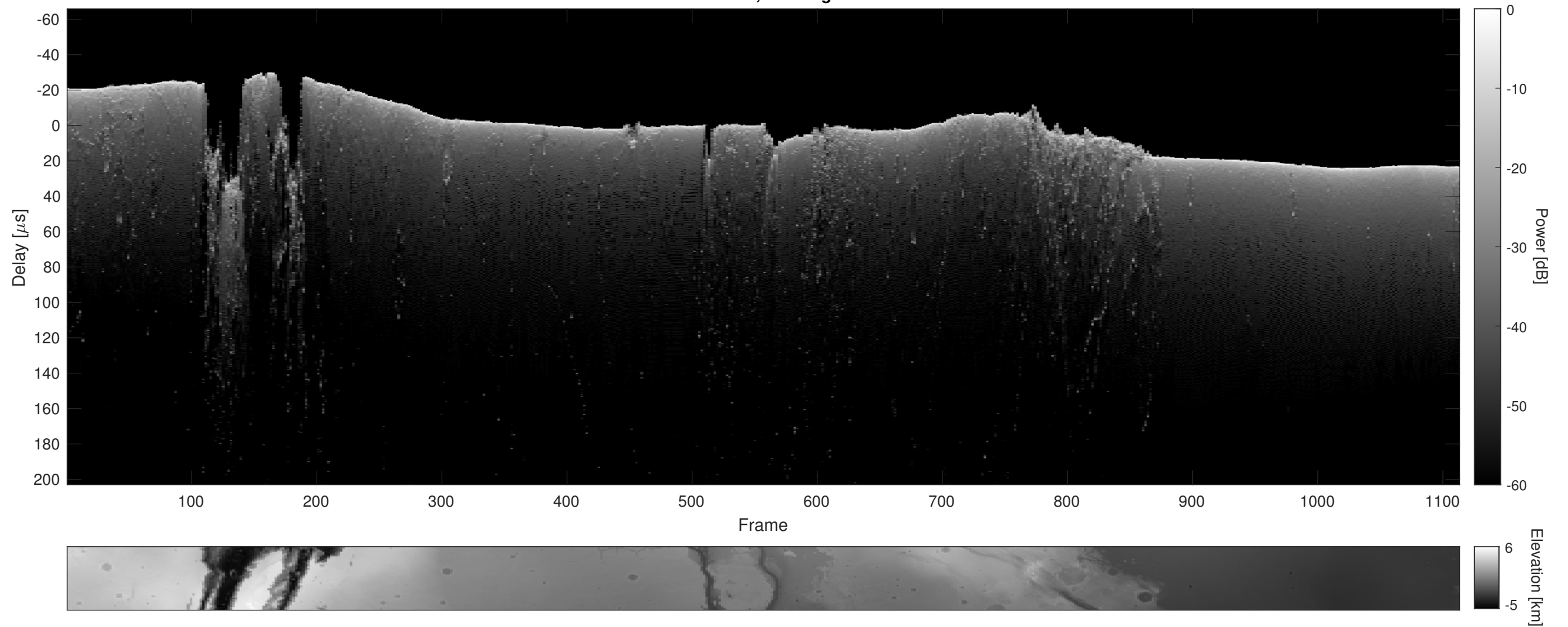
Orbit 22728, Cluttergram
