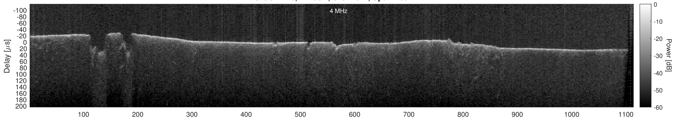
Orbit 22728, Cluttergram
