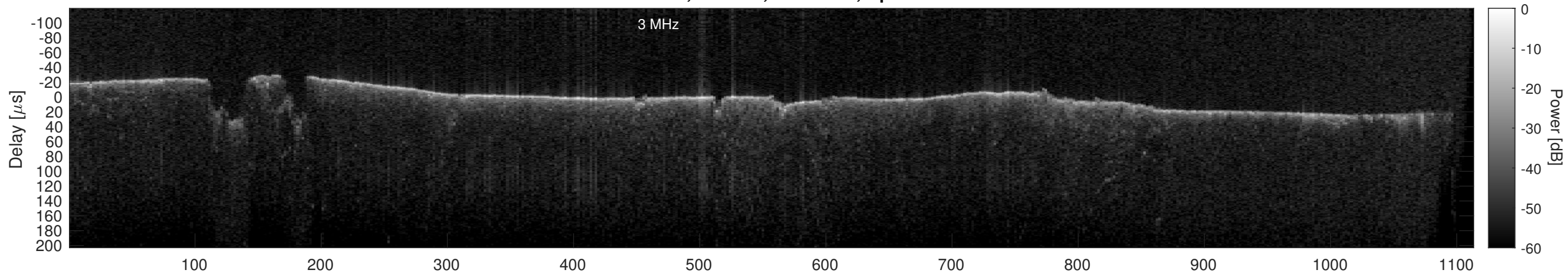
Orbit 22728, Cluttergram
