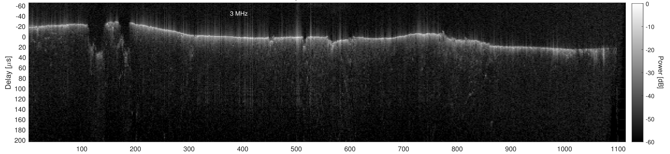
Orbit 22728, Cluttergram
