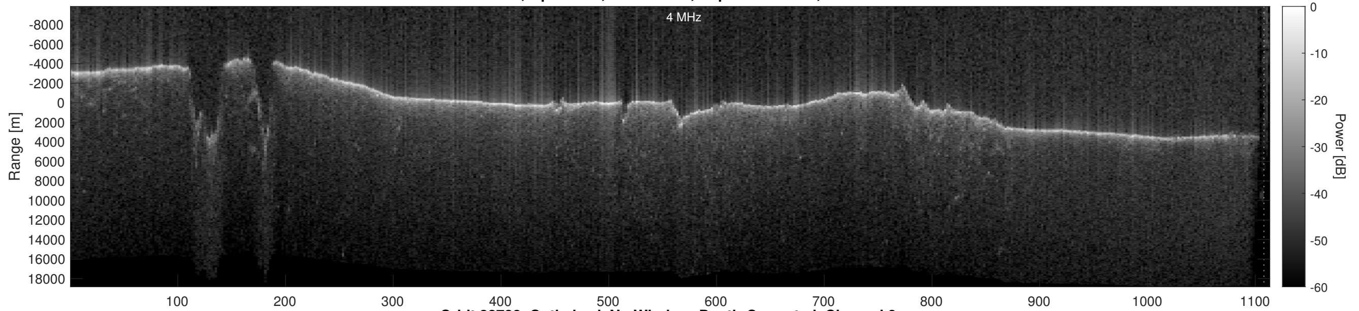
Orbit 22728, Optimized, No Window, Depth-Corrected, Channel 2
