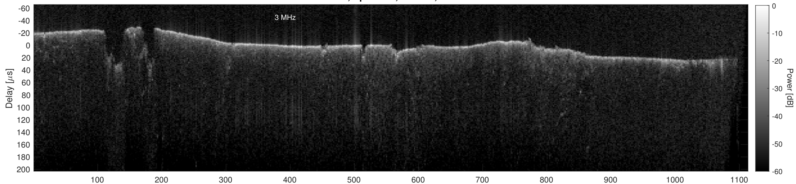
Orbit 22728, Cluttergram
