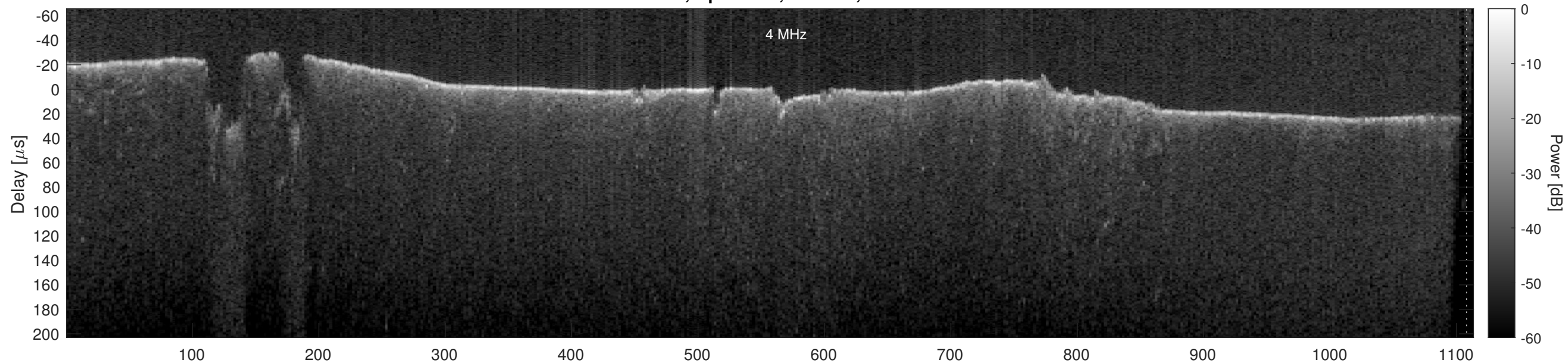
Orbit 22728, Optimized, Window, Channel 2
