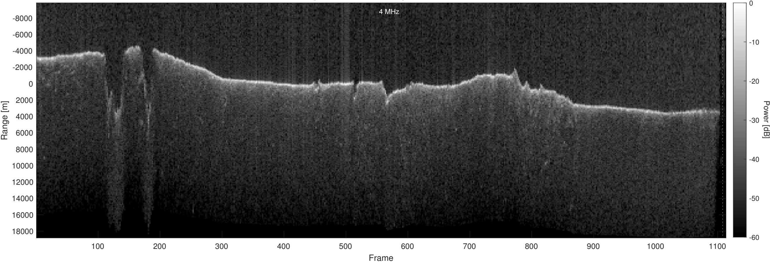
Orbit 22728, Optimized, Window, Depth-Corrected, Channel 2
