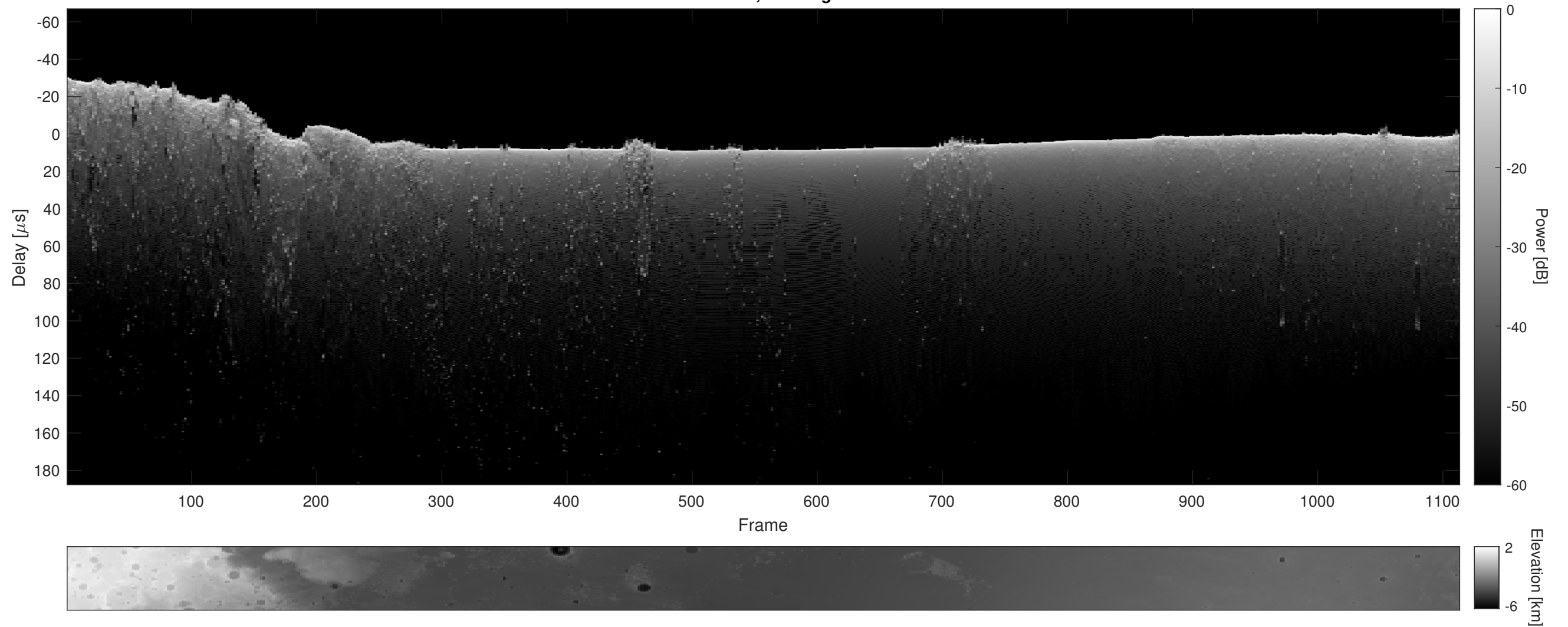
Orbit 22729, Cluttergram
