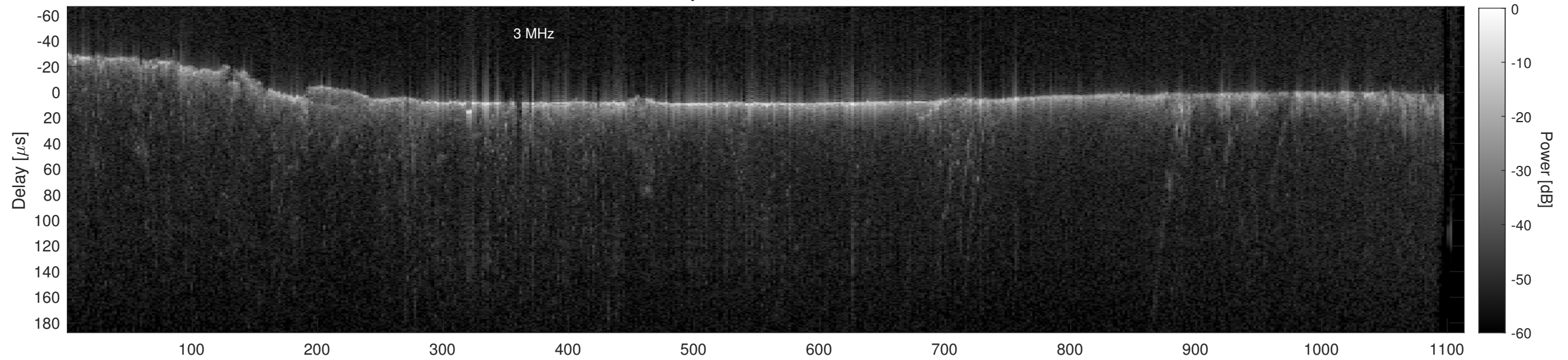
Orbit 22729, Cluttergram
