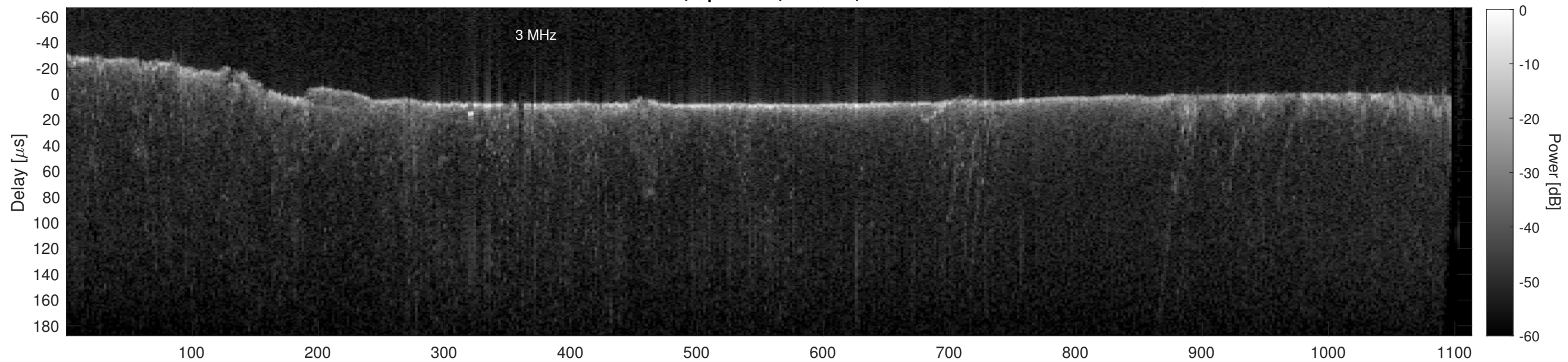
Orbit 22729, Cluttergram
