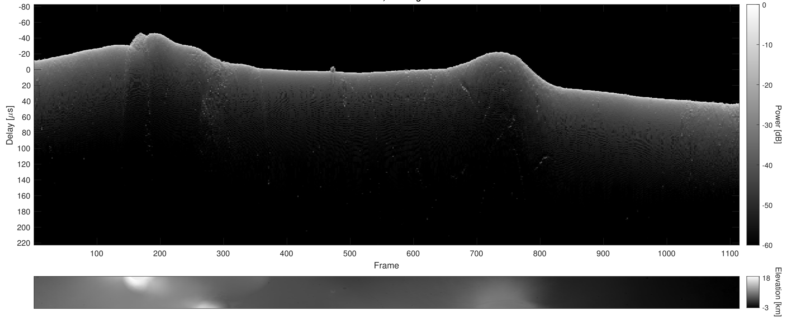
Orbit 22732, Cluttergram
