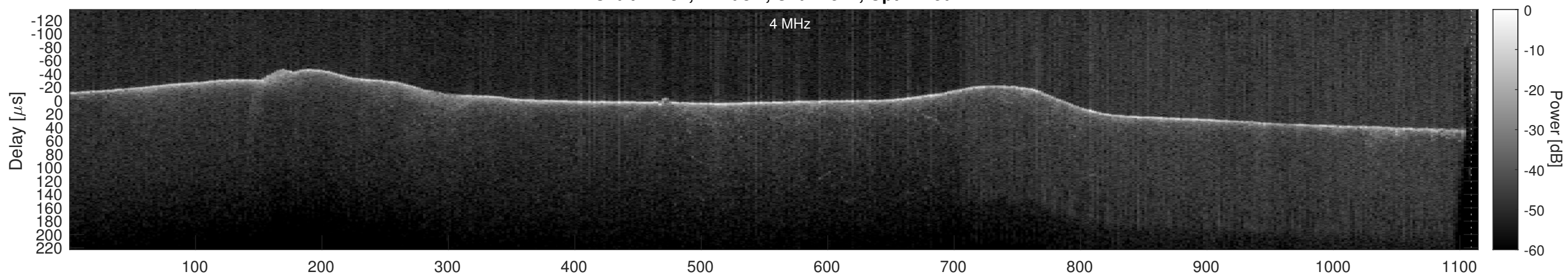
Orbit 22732, Cluttergram
