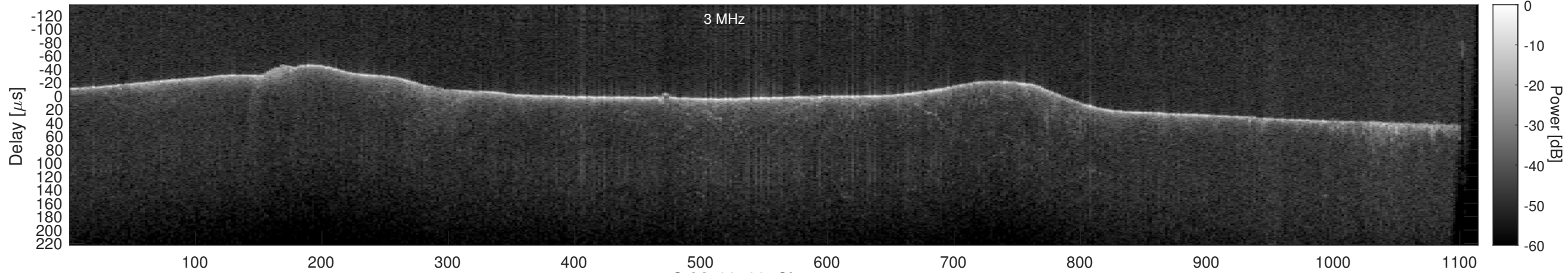
Orbit 22732, Cluttergram
