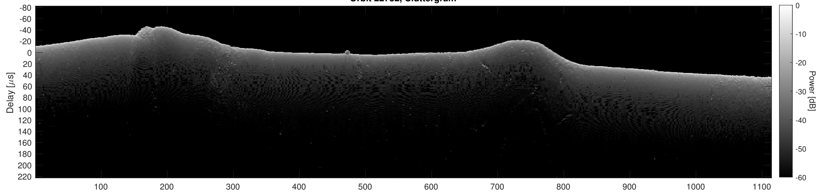
Orbit 22732, Cluttergram
