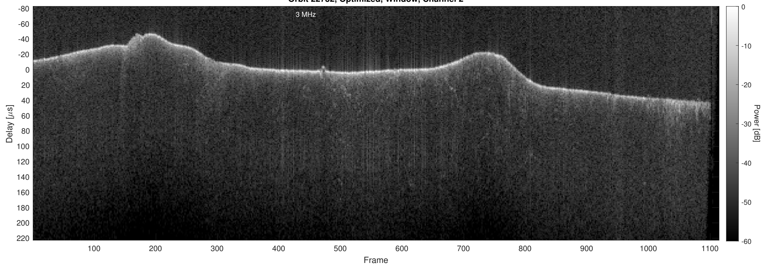
Orbit 22732, Optimized, Window, Channel 2
