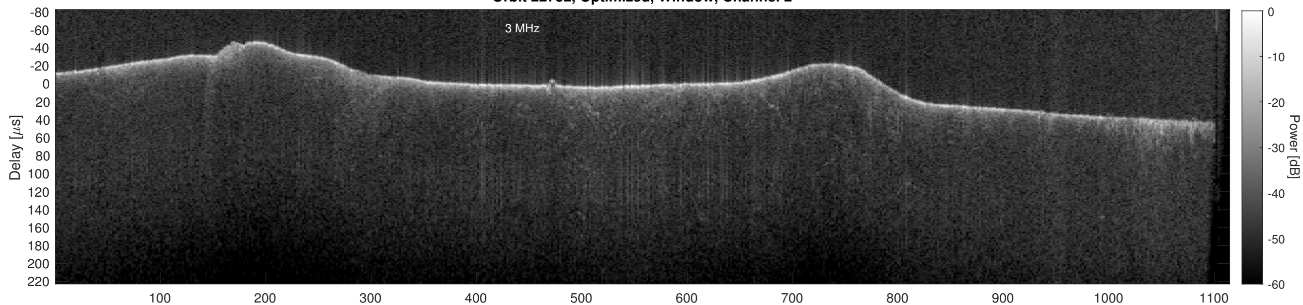
Orbit 22732, Cluttergram
