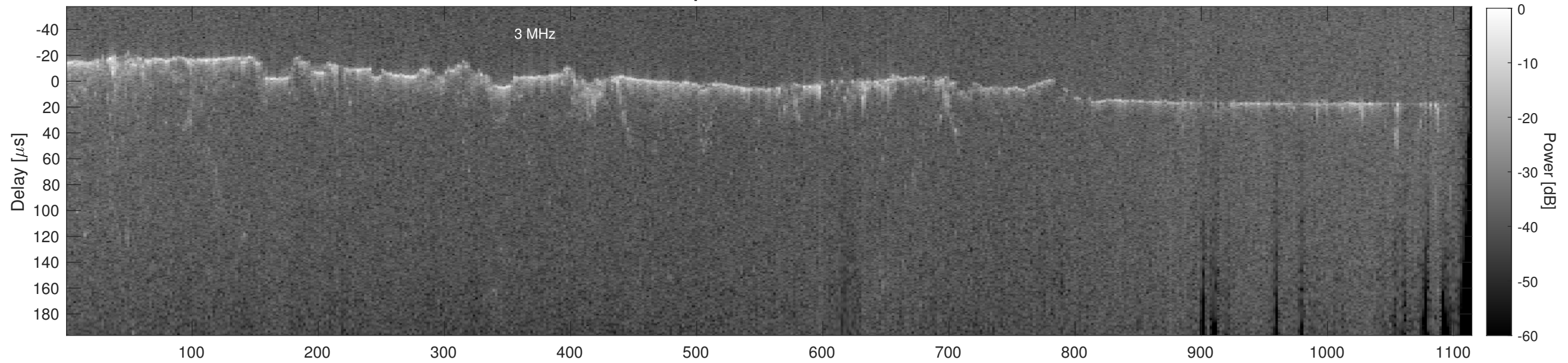
Orbit 22734, Cluttergram
