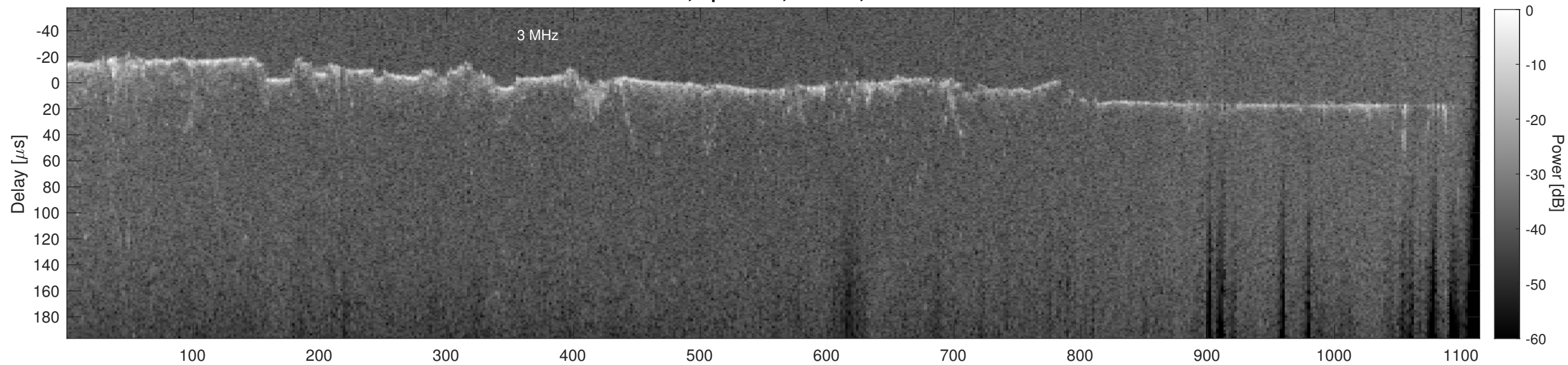
Orbit 22734, Cluttergram
