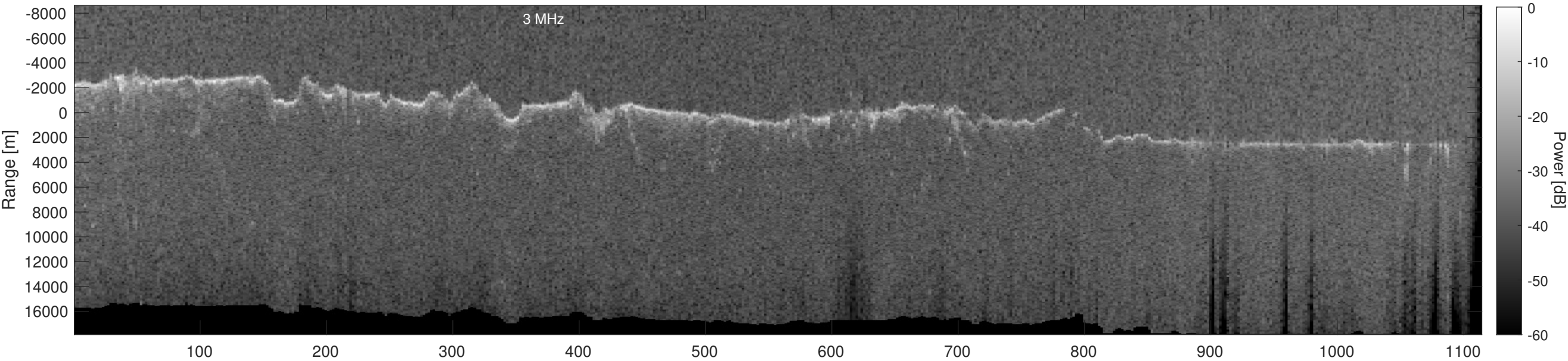
Orbit 22734, Depth-Corrected Cluttergram
