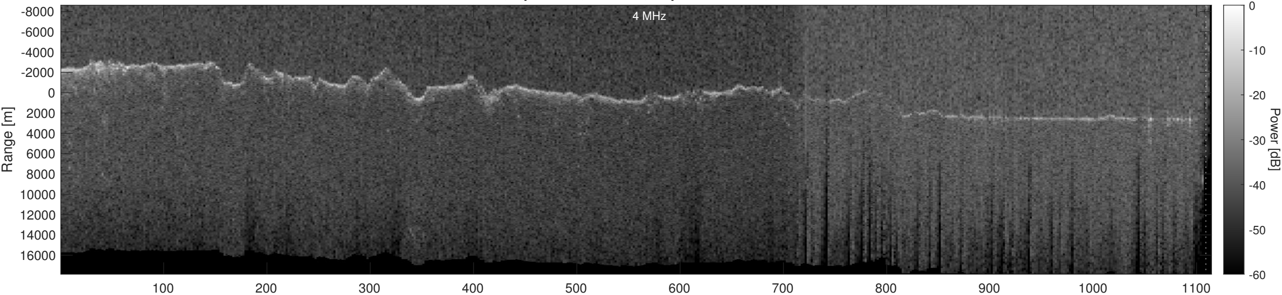
Orbit 22734, Optimized, Window, Depth-Corrected, Channel 2
