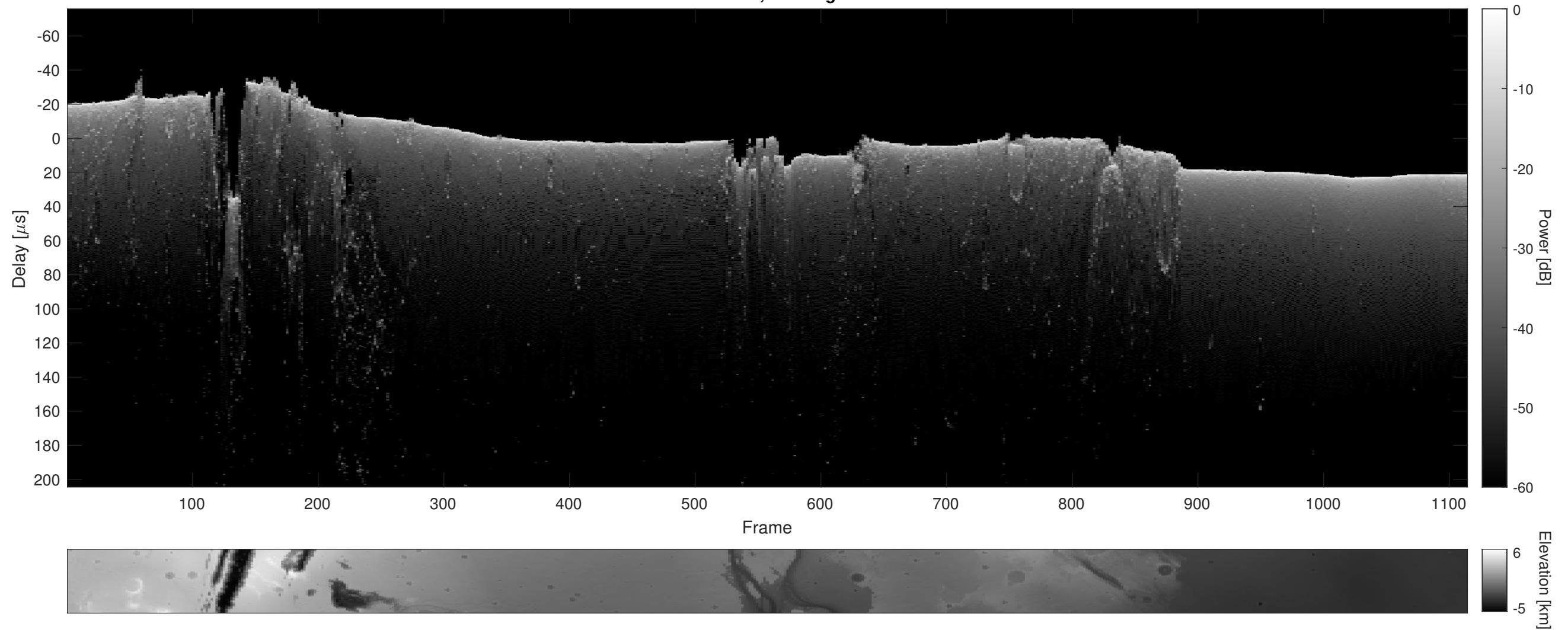
Orbit 22735, Cluttergram
