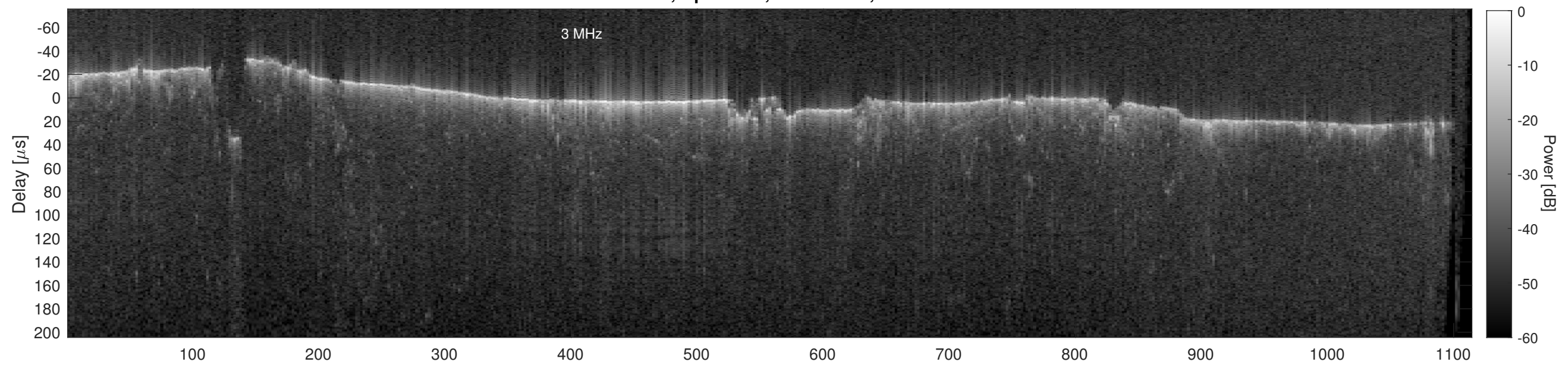
Orbit 22735, Cluttergram
