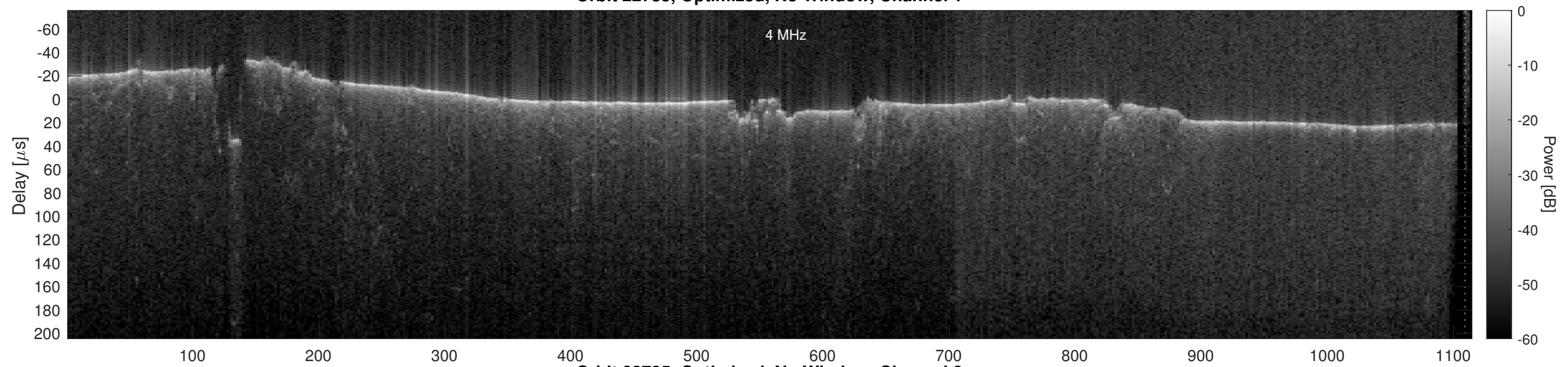
Orbit 22735, Optimized, No Window, Channel 2
