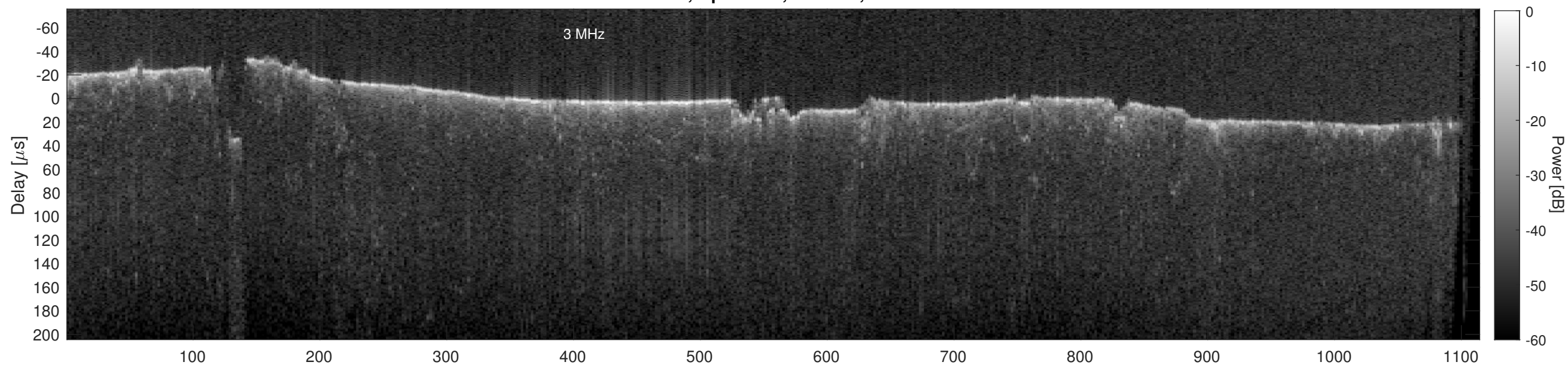
Orbit 22735, Cluttergram
