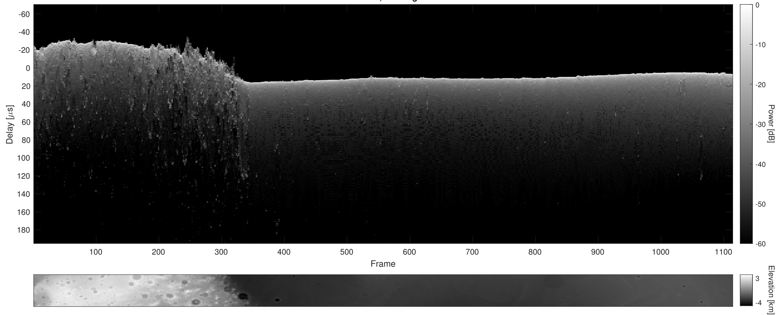
Orbit 22737, Cluttergram
