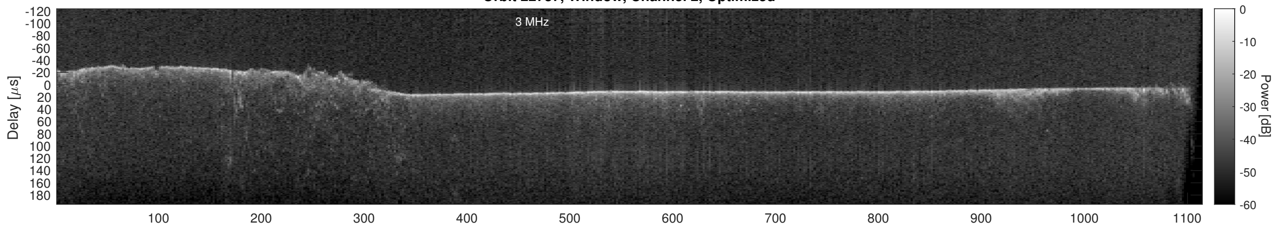
Orbit 22737, Cluttergram
